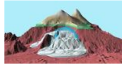
Effects of a flank collapse on Kilauea
