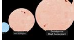
Star Size Comparison
