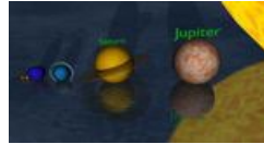
The Universe in 3D: Planet & Star Size Comparison
